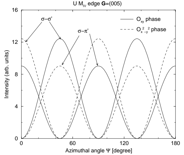
Fig. 5. Azimuthal angle dependence of the RXS peak intensities at \mathbf{G} = (005) near U M_{IV} edge in the AFQ phases. The solid and broken lines represent the results obtained in the O_{xy} and O_{x^2-y^2} orderings within the doublet scheme, respectively. The mixing angle is fixed to being \alpha \simeq 52.48^\circ and both \sigma - \sigma' and \sigma - \pi' channels are shown.
